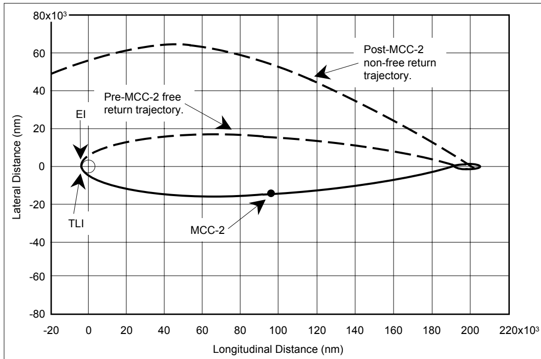
Figure 5. Example of free return (pre MCC-2 burn) and hybrid (post MCC-2 burn) trajectories. 12 The Apollo 13 non-free return Earth perigee was much smaller than the above at 2500 nm.
