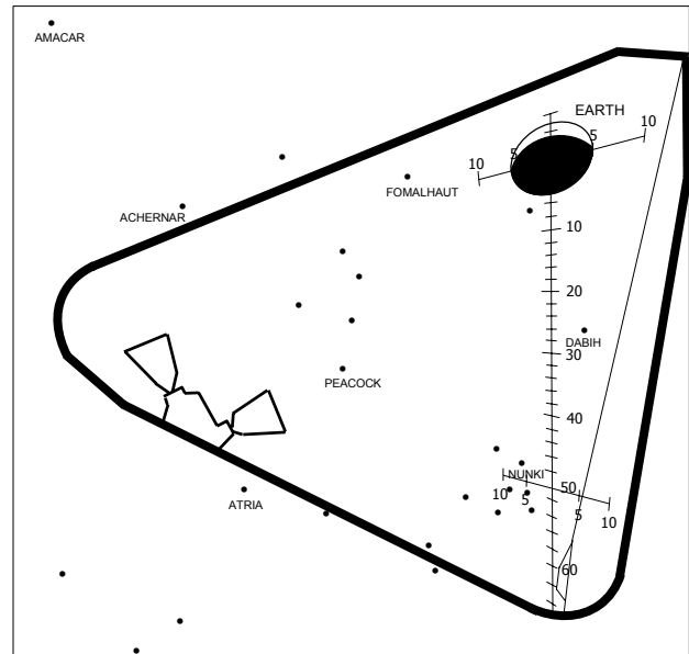
Figure 22. MCC-7 burn LM commander's window view. 28
