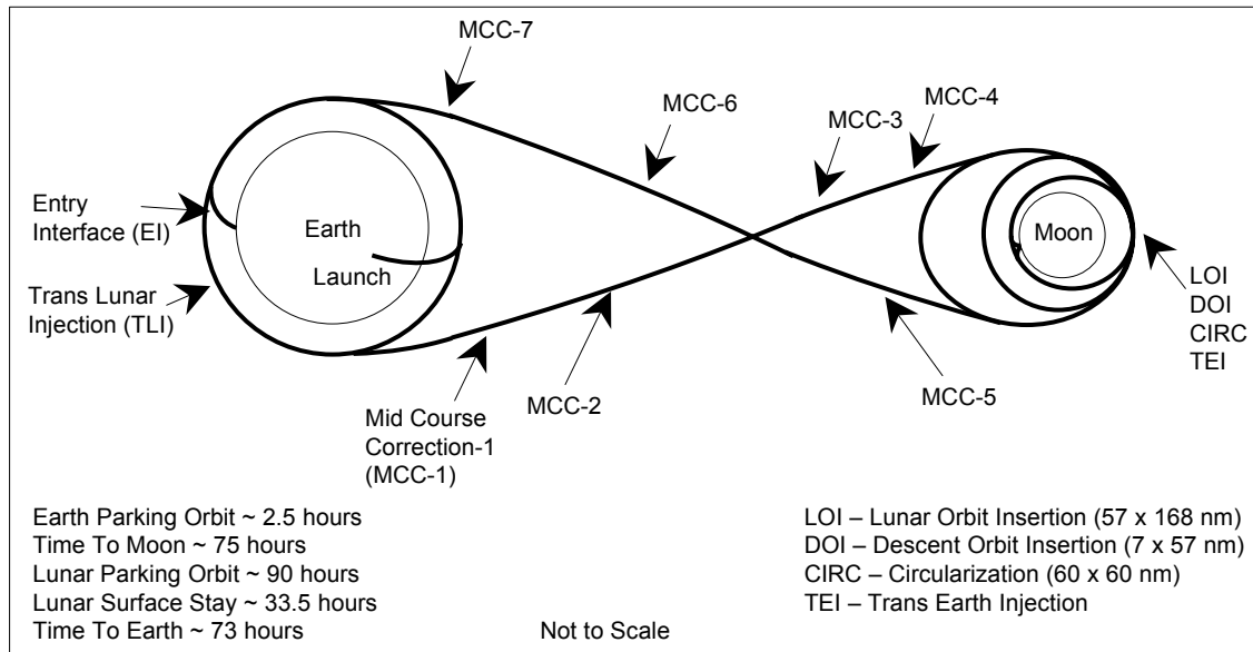
Figure 4. Nominal Apollo 13 mission profile. 12
