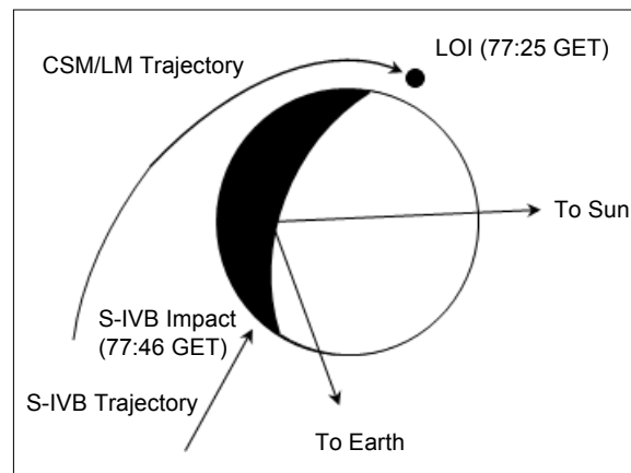
Figure 6. Planned Apollo 13 LOI burn and lunar S-IVB impact. 11
