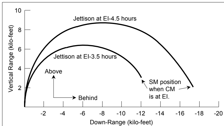
Figure 24. Mission planning plot of Service Module (SM) relative motion after separation from the Lunar Module/Command Module (LM/CM) stack for separation times of EI-3.5 and EI-4.5 hours. 24
