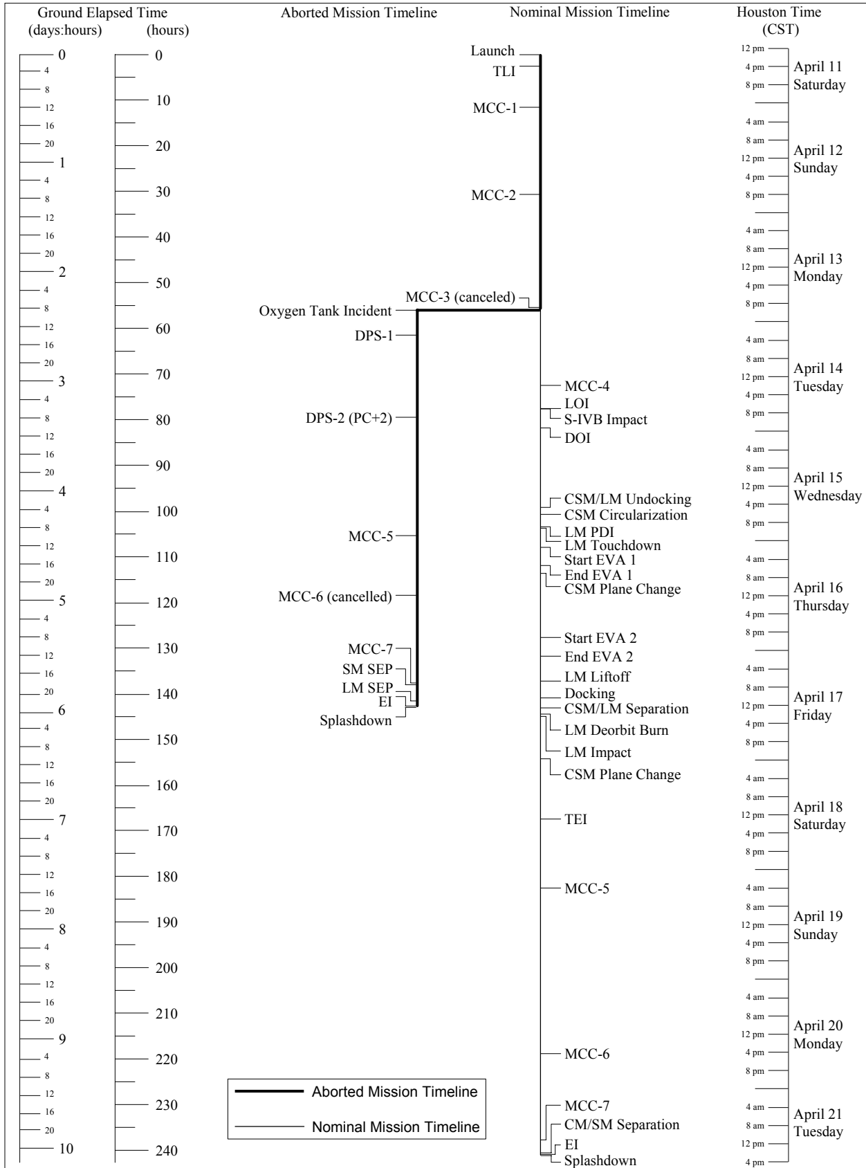
Figure 3. Apollo 13 Aborted Mission and Nominal Mission Timelines
