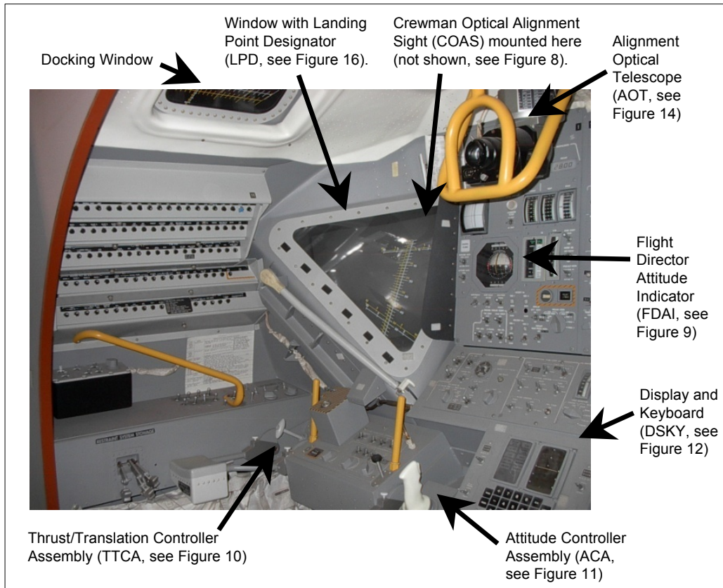
Figure 13. Lunar Module commander's station. The pilot's station (to the right, not shown) was also equipped with a TTCA, ACA, and FDAI.
