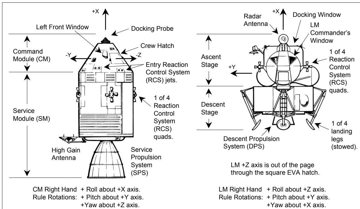
Figure 1. Apollo Command Service Module (CSM) (left) and Lunar Module (LM) (right).
