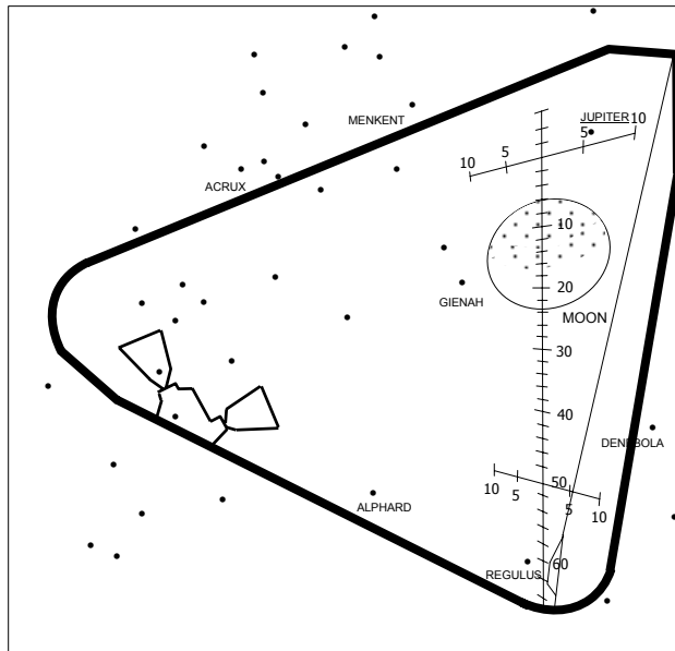
Figure 16. DPS-2 (PC+2) burn LM commander's window view with Landing Point Designator (LPD) scale. 28
