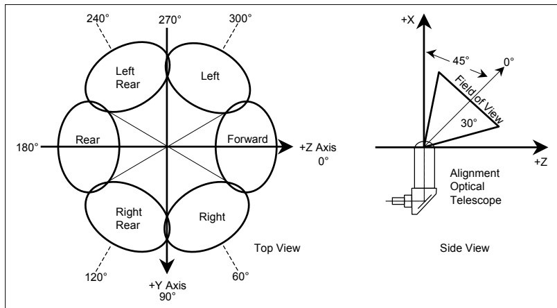
Figure 14. Lunar Module Alignment Optical Telescope (AOT) fields of view. The forward viewing position illustrated in both the top and side views was the only one used during Apollo 13. Axes are the same as those shown in Figure 1.
