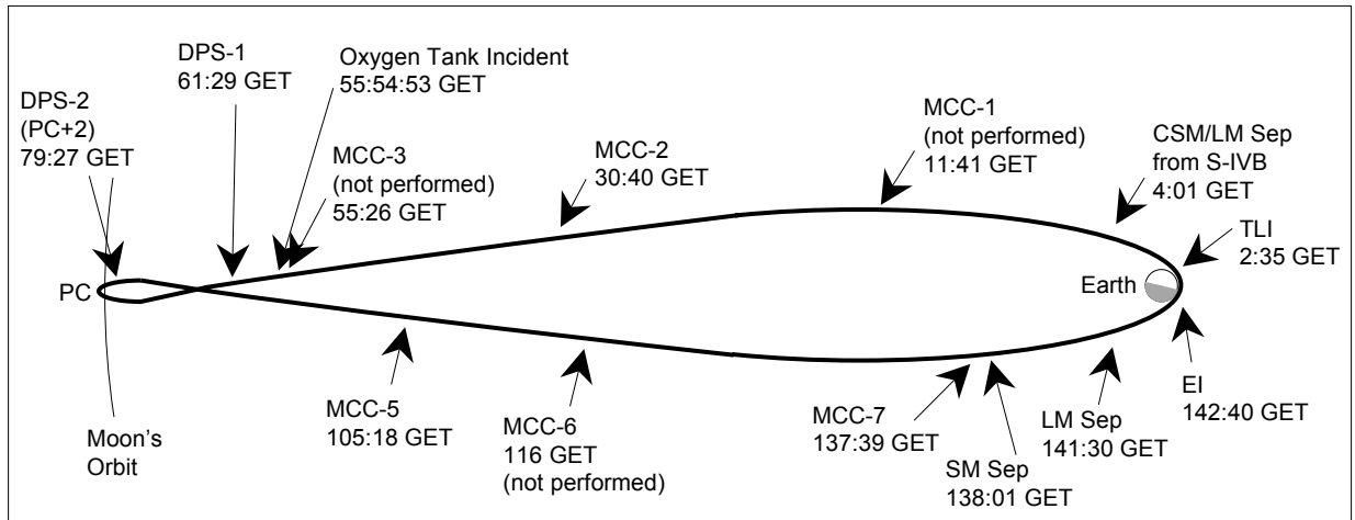
Figure 7. As-flown Apollo 13 trajectory and key events. 17
