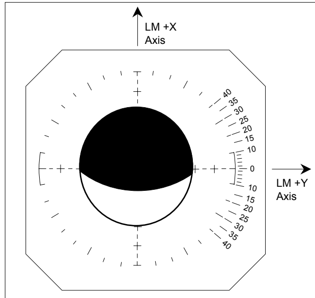
Figure 18. COAS view of Earth for a posigrade trajectory correction burn. 15
