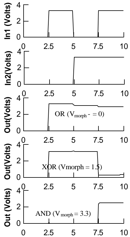
Figure 4 – Evolved Polychromatic circuit exhibiting three different functionalities , OR, XOR and AND.
