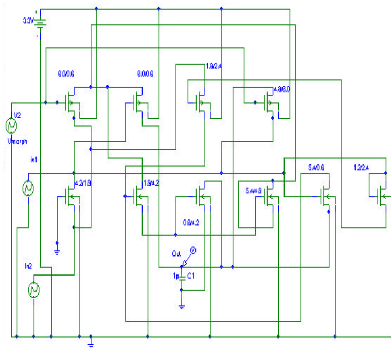
Figure 4 – Evolved Polychromatic circuit exhibiting three different functionalities , OR, XOR and AND.
