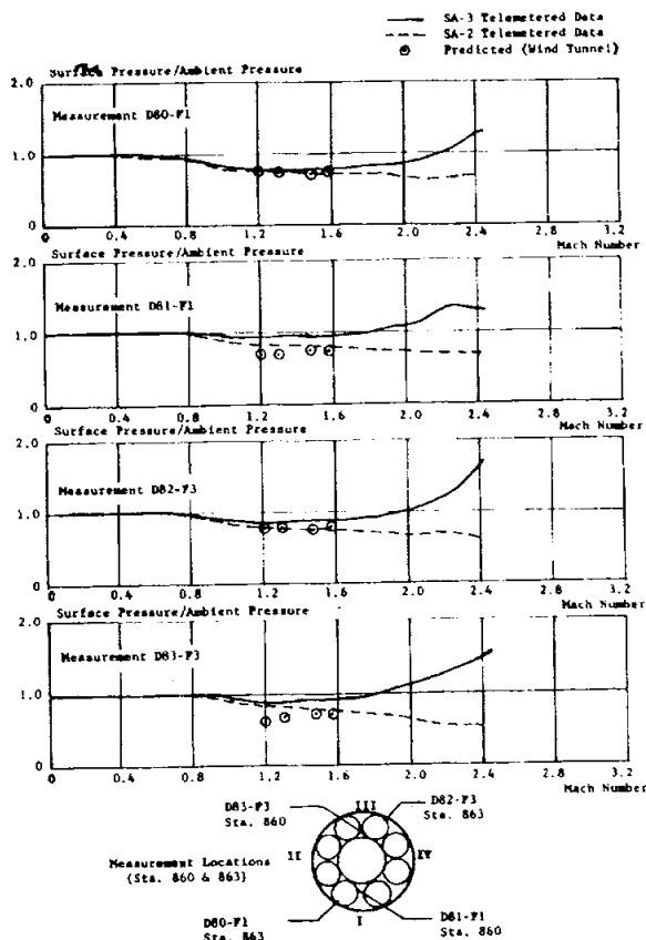
FIGURE 12-4. RATIOS OF SURFACE PRESSURE TO AMBIENT PRESSURE VERSUS MACH NUMBER
