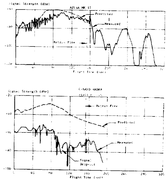
FIGURE 13-4. AZUSA AND RADAR SIGNAL STRENGTH
