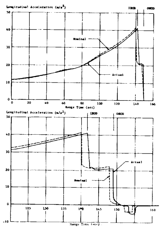
FIGURE 4-4. LONGITUDINAL ACCELERATION
