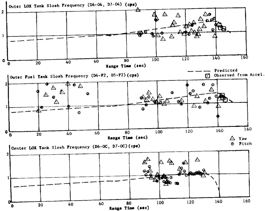
FIGURE 7-17. SLOSHING FREQUENCIES
