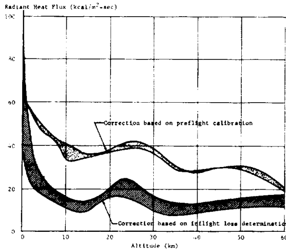
FIGURE 11-9. RADIANT HEATING RATES FOR SA-3 FLIGHT COMPARING PREFLIGHT AND INFLIGHT DATA CORRECTION TECHNIQUES
