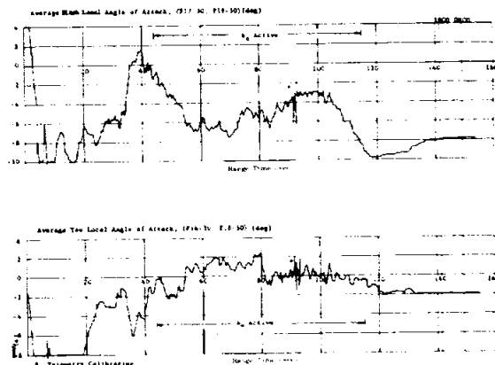
FIGURE 7-11. PITCH AND YAW LOCAL ANGLES-OF-ATTACH
