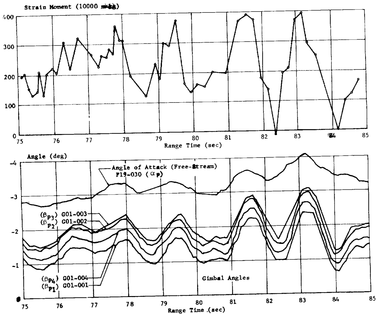
FIGURE 10-2. BENDING MOMENT AT STATION 979, ANGLE-OF-ATTACK, AND GIMBAL ANGLE VERSUS RANGE TIME
