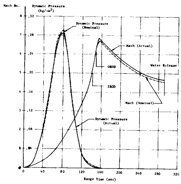
FIGURE 4-3. DYNAMIC PRESSURE AND MACH NUMBER
