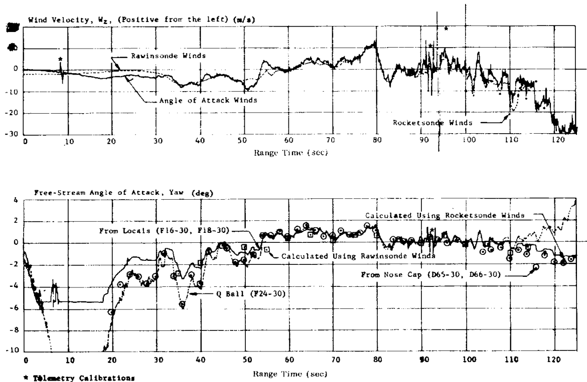
FIGURE 7-6. YAW PLANE WIND COMPONENT AND FREE-STREAM ANGLE-OF-ATTACK
