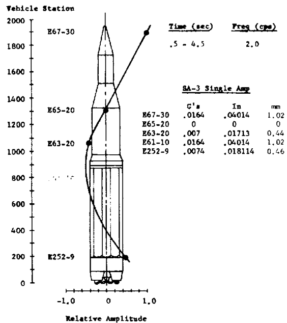
FIGURE 10-6. SA-3 BENDING MODE - FIRST MODE, YAW AT LIFTOFF
