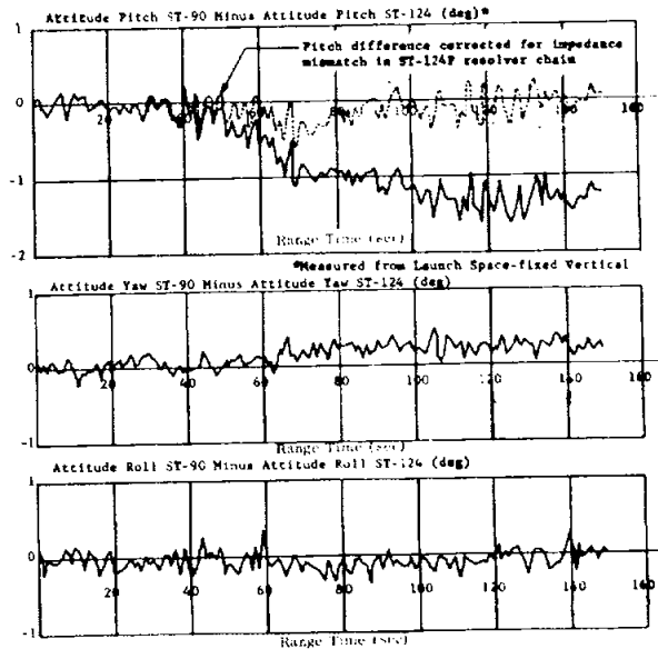
FIGURE 7-15. ATTITUDE DIFFERENCES BETWEEN ST-90 AND ST-124P
