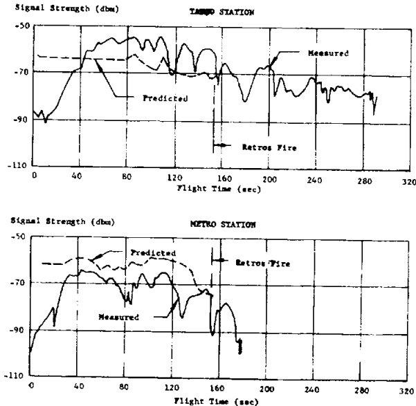
FIGURE 13-3. UDOP SIGNAL STRENGTH
