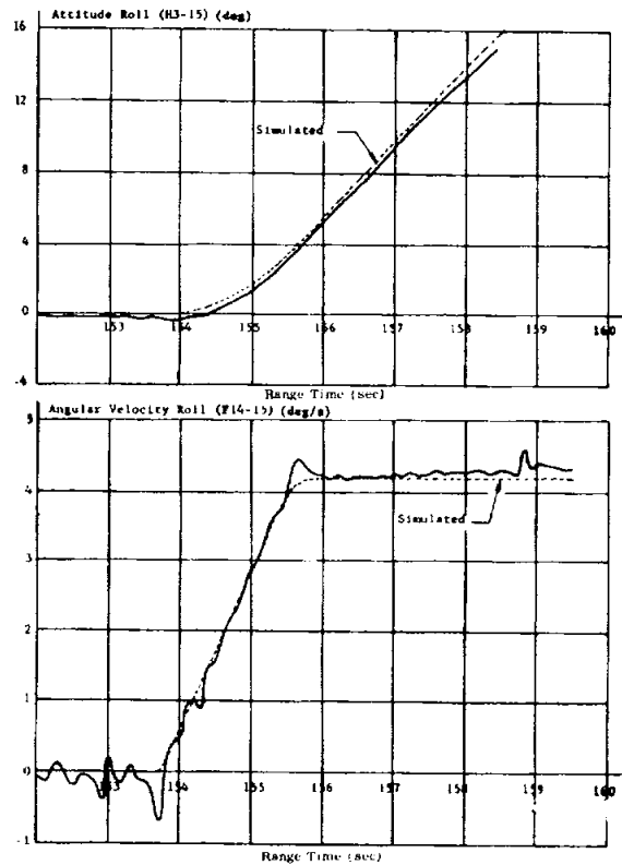
FIGURE 7-9. ROLL DURING RETRO ROCKET FIRING
