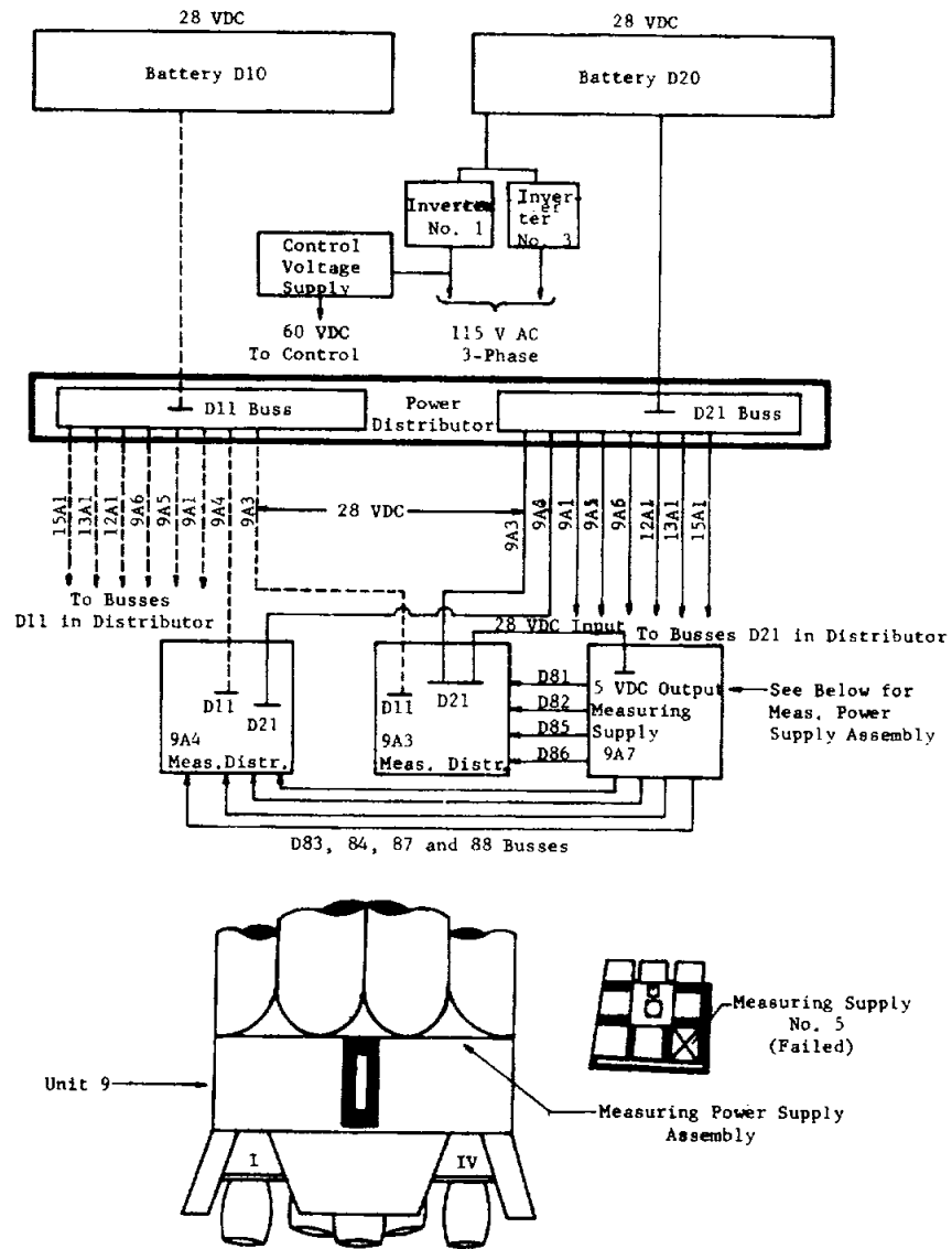
FIGURE 9-1. DISTRIBUTOR CONNECTIONS AND UNIT 9 MEASURING SUPPLY
