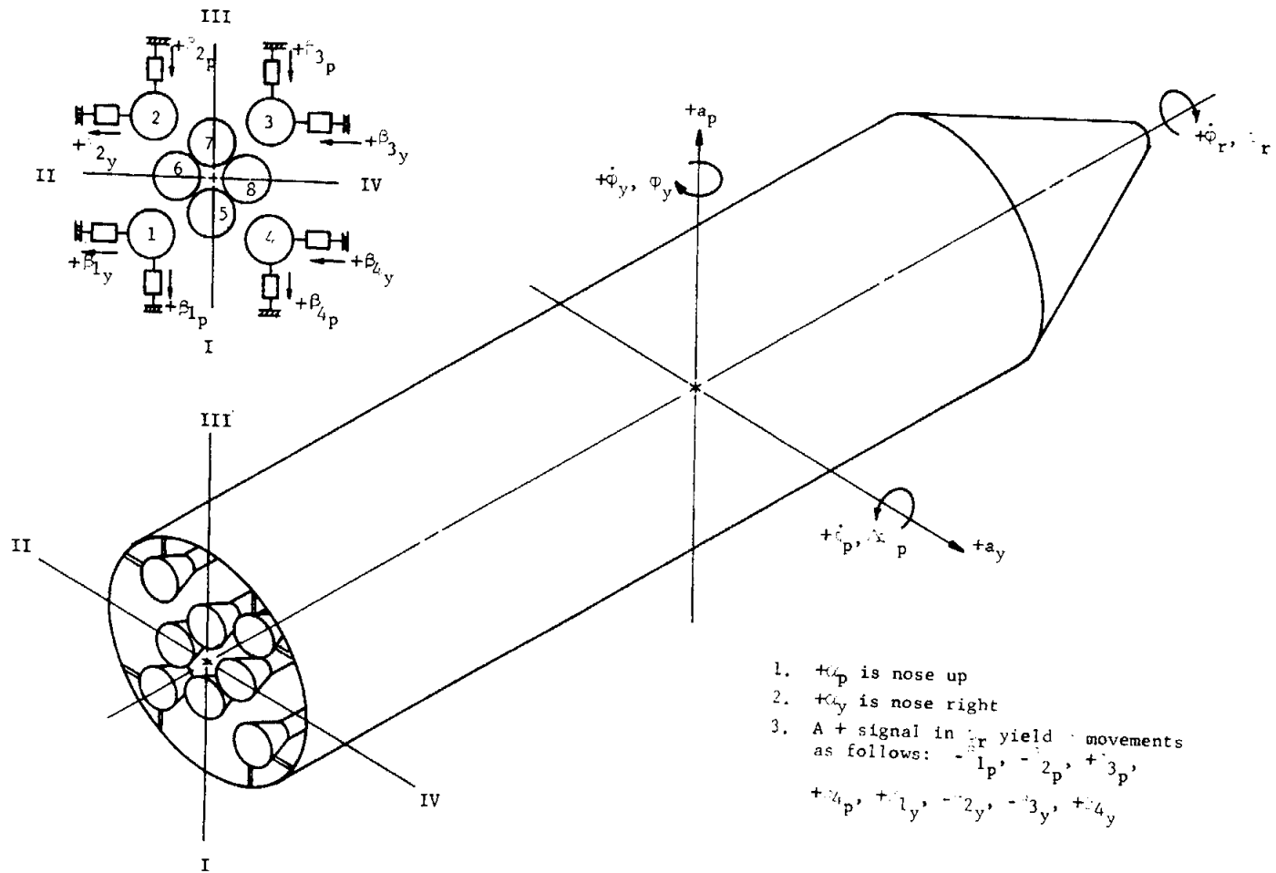
FIGURE 1-1. SATURN BOOSTER POLARITY CHART
