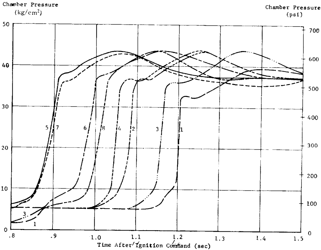
FIGURE 5-3. CHAMBER PRESSURE BUILDUP
