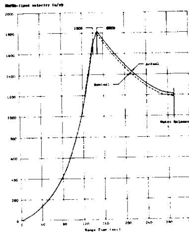
FIGURE 4-2. EARTH-FIXED VELOCITY
