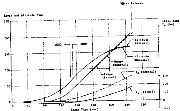
FIGURE 4-1. TRAJECTORY
