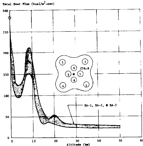
FIGURE 11-8. TOTAL HEATING RATE ON FLAME SHIELD, SA-1, SA-2 AND SA-3
