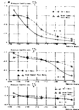
FIGURE 12-7. PRESSURE COEFFICIENT VERSUS VEHICLE STATION AT VARIOUS MACH NUMBERS ON CENTAUR - SIMULATION PANEL I
