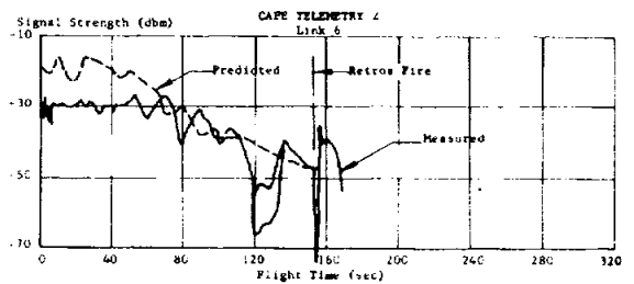
FIGURE 13-1. TELEMETRY SIGNAL STRENGTH (CAPE TELEMETRY 2)
