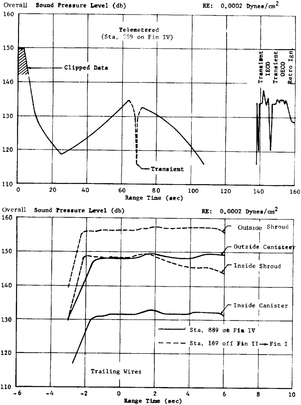
FIGURE 10-10. SA-3 VEHICLE ACOUSTICS
