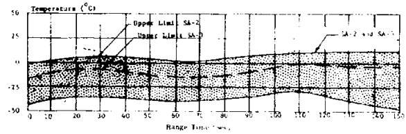
FIGURE 11-10. ENGINE COMPARTMENT STRUCTURAL TEMPERATURES
