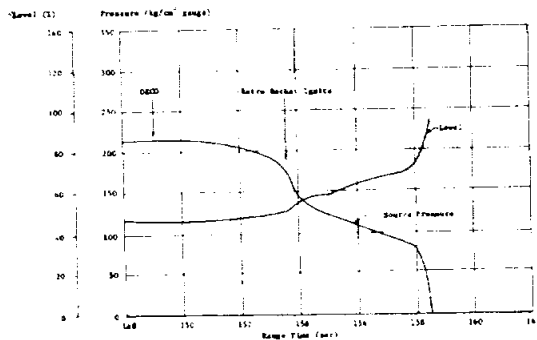
FIGURE 7-14. HYDRAULIC SOURCE PRESSURE AND LEVEL
