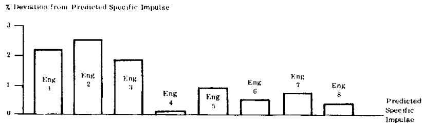
FIGURE 5-2. INDIVIDUAL ENGINE DEVIATION FROM PREDICTED SPECIFIC IMPULSE
