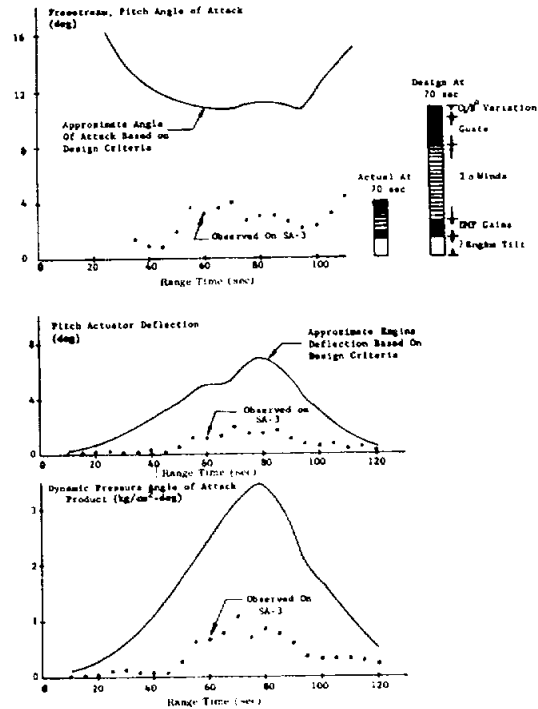
FIGURE 7-4. PITCH ANGLE DESIGN CRITERIA (8 ENGINES OPERATING WITH 7 ENGINE TILT PROGRAM)
