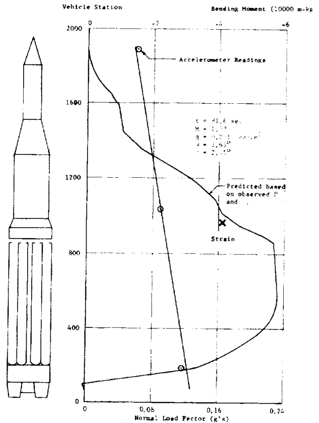
FIGURE 10-1. BENDING MOMENT AND NORMAL LOAD FACTOR
