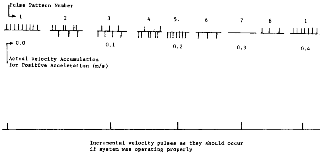
FIGURE 8-4. INCREMENTAL VELOCITY PULSE PATTERNS, ST-124P CROSS RANGE
