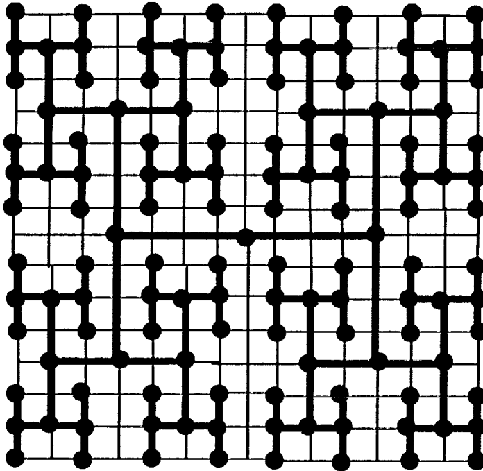
Fig. 3.5. An H-tree embedding of a T_7 on an M_{15} .
