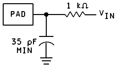
CIRCUIT A
